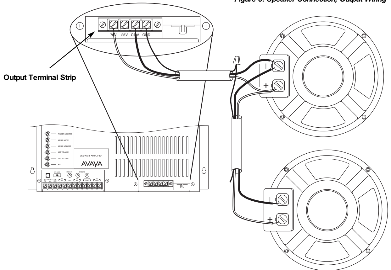
Figure 8: Speaker Connection, Output Wiring
