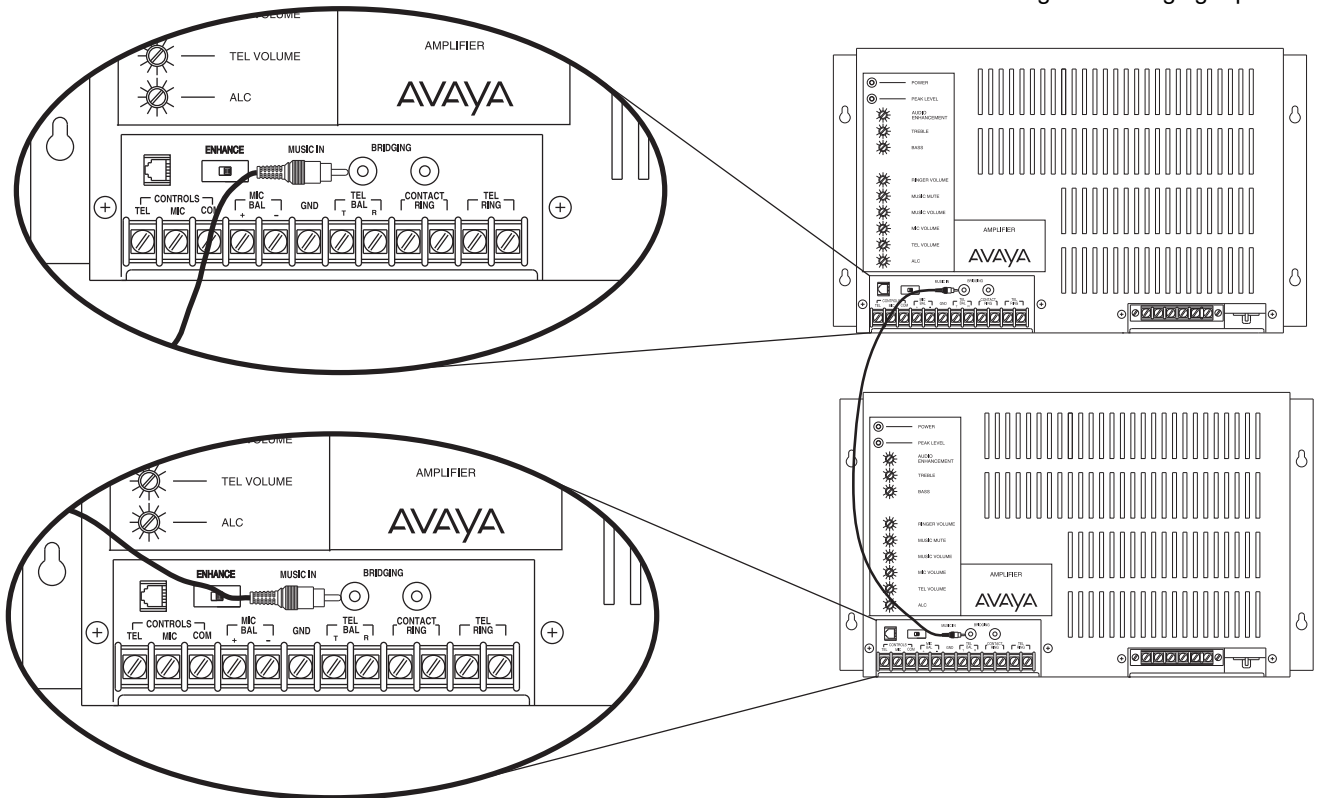
Figure 6: Bridging Inputs
